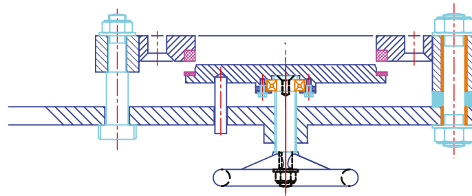
VIEW ON VALVE - CLOSED
