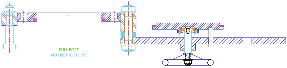
VIEW ON VALVE - OPEN
